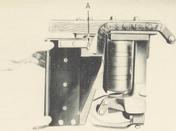
First: Raise Arc Chute to unhook catch (A) at top of Contactor
